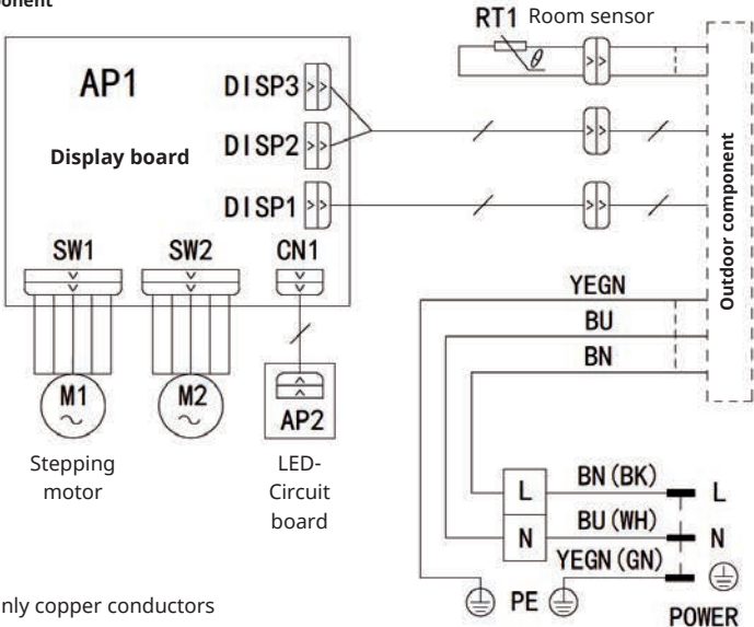
Indoor component
